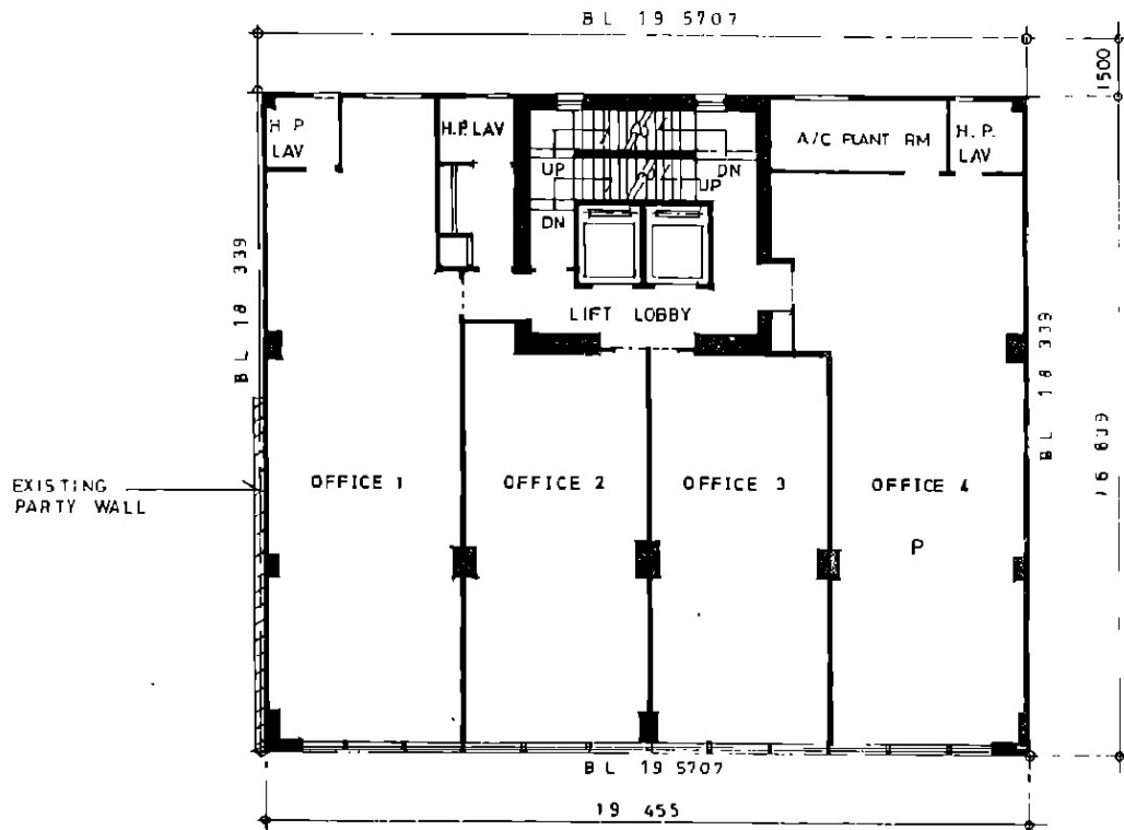
2nd - 3rd FLOOR PLAN
